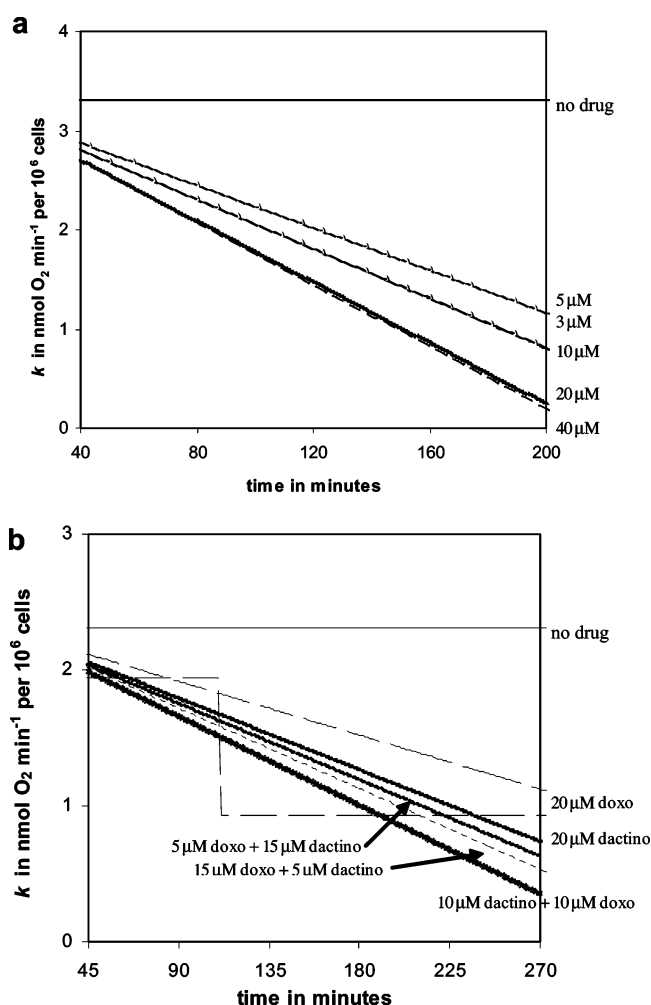
Figure 8. Respiration rate constants, k , calculated from plots of [\text{O}_2] vs t by fitting the data to the quadratic form \alpha + \beta t + \gamma t^2 , differentiating with respect to t , dividing by the number of cells, and multiplying by the reaction volume. All curves have been normalized to give the same k at t = 0 , the value obtained in the absence of the drug. (a) Values of k obtained for cells exposed to various [dactinomycin] (Figure 2a and b). From top to bottom, the plots correspond to [dactinomycin] = 0, 5, 3, 10, 40, and 20 \mu\text{M} ; the curves for 5 and 3 \mu\text{M} , and those for 20 and 40 \mu\text{M} , are virtually indistinguishable. (b) Values of k obtained for cells exposed to 20 \mu\text{M} drug (Figure 6). From top to bottom: no drug, 20 \mu\text{M} doxorubicin, 20 \mu\text{M} dactinomycin, 15 \mu\text{M} dactinomycin + 5 \mu\text{M} doxorubicin, 5 \mu\text{M} dactinomycin + 15 \mu\text{M} doxorubicin, and 10 \mu\text{M} dactinomycin + 10 \mu\text{M} doxorubicin. The step function is the k value obtained by fitting the [\text{O}_2] results for 20 \mu\text{M} doxorubicin to two straight lines.
